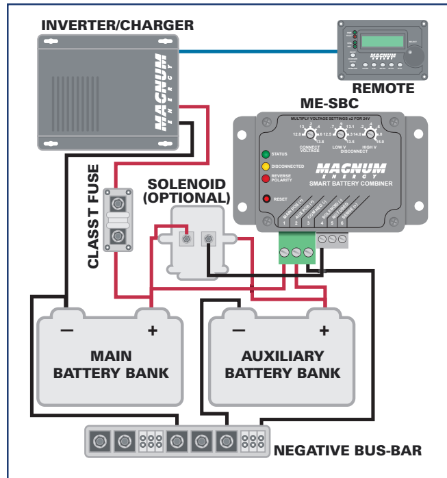
Solenoid Drive
